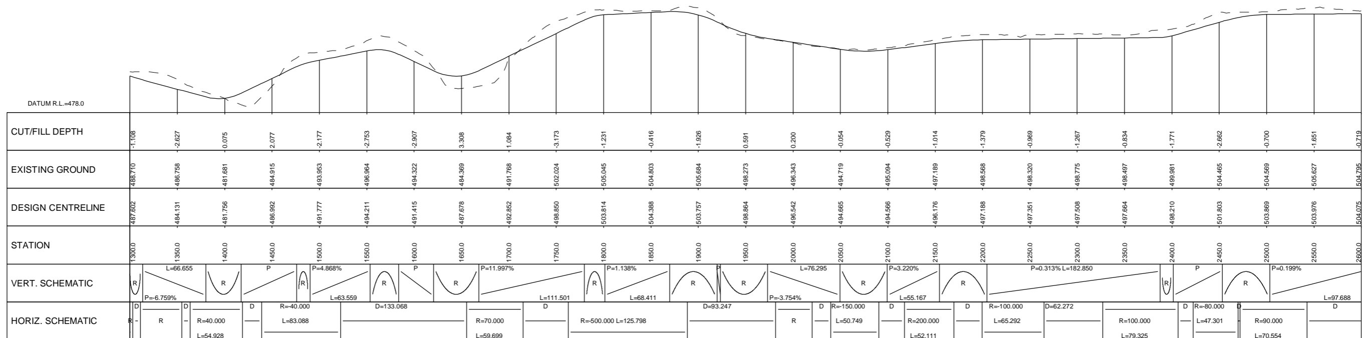
LONG SECTION SCALE 1:2000 Hz 1:500 Vt
