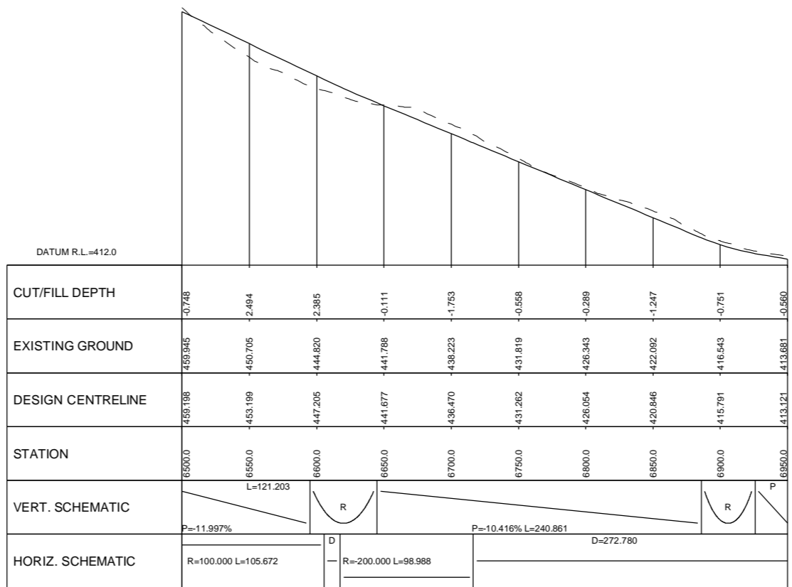
LONG SECTION SCALE 1:2000 Hz 1:500 Vt
